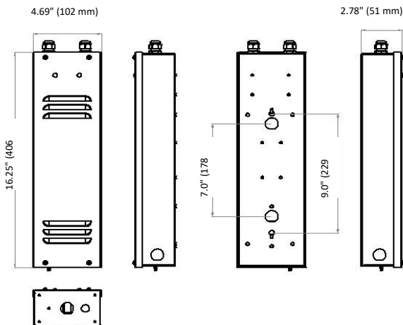
BALLAST BOX (SINGLE or DOUBLE)
